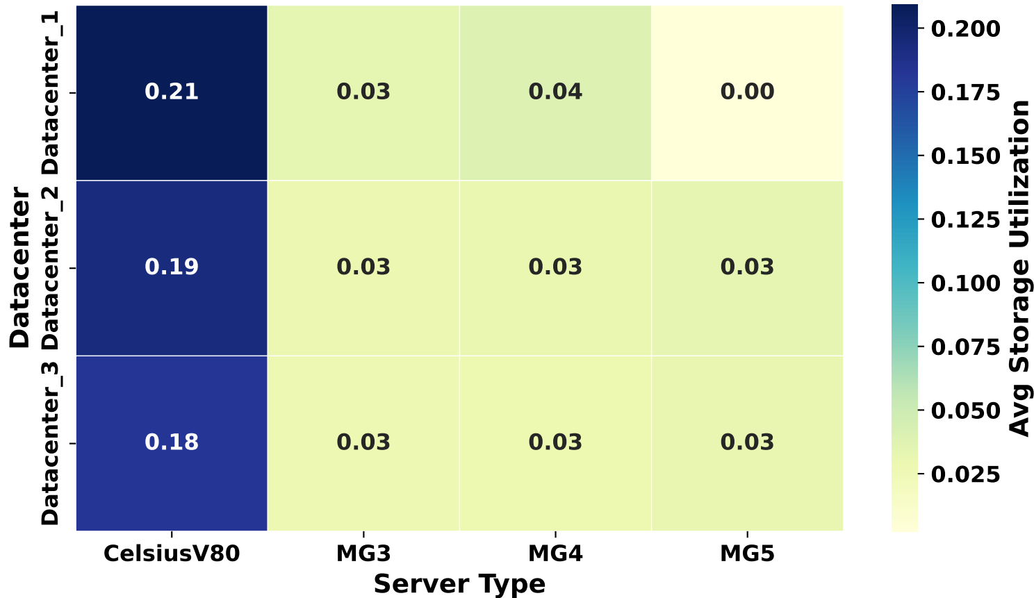
Mean Storage Utilization
